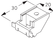
SG 3603 Bracket
