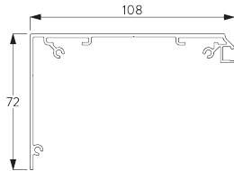
SG 11530 Installation profile fascia 110 mm
