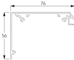
SG 11430 Installation profile fascia 73 mm
