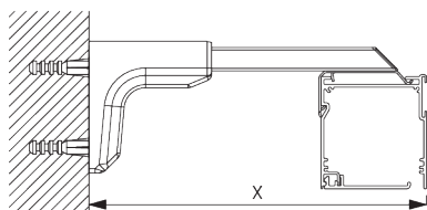
Universal Smart Fix SG 11154 - SG 11156 and bracket SG 2521:
