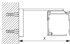
Smart Fix SG 11200 - SG 11204 and bracket SG 2521:
