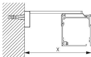
Square Smart Fix SG 11210 - SG 11214 and bracket SG 2521:
