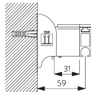
For parallel fixing of profile to the wall
