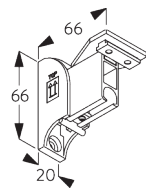
SG 6668 Wall bracket
