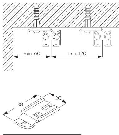
SG 3832 Bracket
