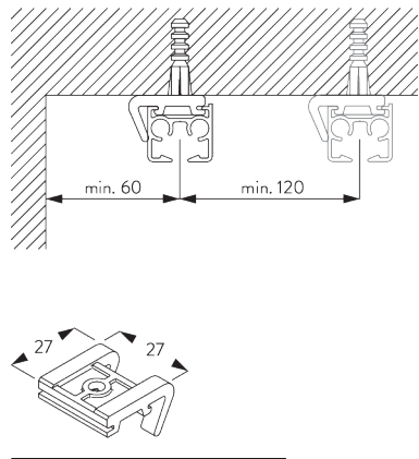
SG 3826 Bracket
